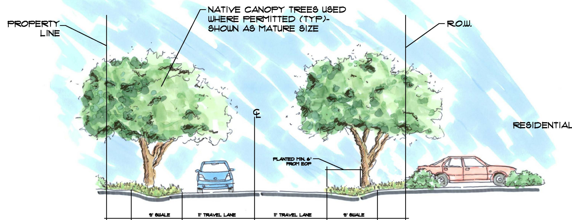
TYP. STREET SECTION
